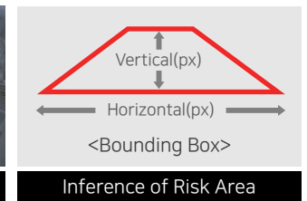
Forward Detection
